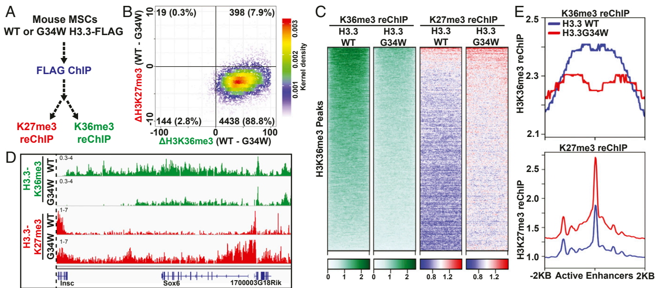
Fig. 2. Local loss of H3K36me3 and gain of H3K27me3 in cells expressing H3.3G34W. (A) Strategy used to identify local changes in H3K27me3 and H3K36me3 in cells expressing H3.3 WT or G34W in vivo. (B) Scatterplot displaying the correlation between loss of H3.3X-K36me3 and gain of H3.3X-K27me3 at H3K36me3-enriched peaks. Each point represents a H3K36me3 peak, and the difference in the number of normalized ChIP-Seq reads was plotted. (C) Heatmap displaying the enrichment of H3.3-K36me3 and H3.3-K27me3 reChIP enrichment at H3K36me3 peaks in cells expressing H3.3 WT or G34W. (D) Genome browser view of the Sox6 gene displaying the loss of H3.3X-K36me3 and gain of H3.3X-K27me3. (E) Metagenesis analysis showing the average profile of H3.3X-K36me3 and H3.3X-K27me3 reChIP at active enhancers (promoter-distal H3K27ac peaks) in cells expressing H3.3 WT or G34W.
