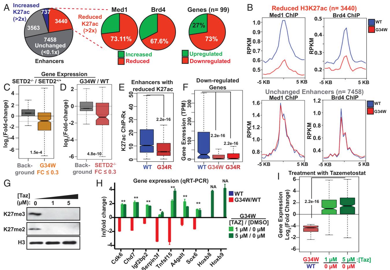
Fig. 4. Reduced gene enhancer activity in cells expressing H3.3 G34W. (A) Pie chart displaying the proportion of enhancers with reduced H3K27ac ( \Delta K27ac \leq 2), unchanged ( 0.9 \leq \Delta K27ac \leq 1.1) and increased H3K27ac ( \Delta K27ac \geq 2) in H3.3 G34W-expressing cells. (Right) Pie chart displaying the changes in Med1/Brd4 occupancy at enhancers with reduced H3K27ac and expression of genes associated with them. Gene-enhancer associations were identified using GREAT and genes associated with at least three enhancers with reduced H3K27ac ( n = 99 ) were used for the analyses. (B) Average profiles of Med1 (Left) and Brd4 ChIP-Seq (Right) displaying their average profiles at enhancers with decreased H3K27ac (Top, n = 3,440 ) and unchanged enhancers (Bottom, n = 7,458 ). (C) Boxplot displaying the change in the expression of H3.3 G34W down-regulated genes (fold change \leq 0.3, n = 279 ) in SETD2 -/- cells. Dashed line displays a twofold change. (D) Boxplot displaying the change in the expression of genes down-regulated by SETD2 knockout (fold change \leq 0.3, n = 132 ) in cells expressing H3.3G34W. Dashed line displays a twofold change. (E) Boxplot displaying the H3K27ac enrichment at enhancers with reduced H3K27ac (as defined in Fig. 3A) in cells expressing H3.3 WT or G34R. (F) Boxplot displaying the expression of H3.3 G34W down-regulated genes (fold change \leq 0.3, n = 279 ). TPM, transcripts per million. (G) Immunoblots of whole cell extracts from cells expressing H3.3G34W treated with 0 \mu M, 1 \mu M, or 5 \mu M tazemetostat. (H) Fold change in the expression of genes down-regulated by the expression of H3.3G34W. Samples treated G34W/WT (red), cells expressing H3.3G34W treated with tazemetostat 1 \mu M/0 \mu M (light green) and 5 \mu M/0 \mu M (dark green) as measured by RT-qPCR. (I) Boxplots displaying the fold change in the expression of genes down-regulated by the expression of H3.3G34W (FC \leq 0.3, n = 279 ) in the same samples as shown in H. Center line in the boxplots represents the median; Bottom and Top of the box represent 25th and 75th quartiles; whiskers extend to 1.5 \times interquartile range. Background includes all genes with posterior probability of differential expression (PPDE) \geq 0.95. P value was determined using Wilcoxon's rank sum test.
